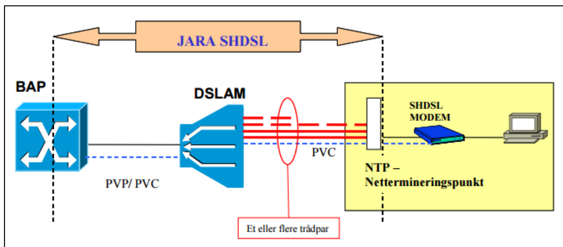
Figure 25: Reference figure Jara SHDSL.
