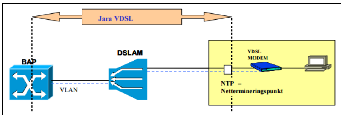
Figure 24: Reference figure Jara VDSL.
